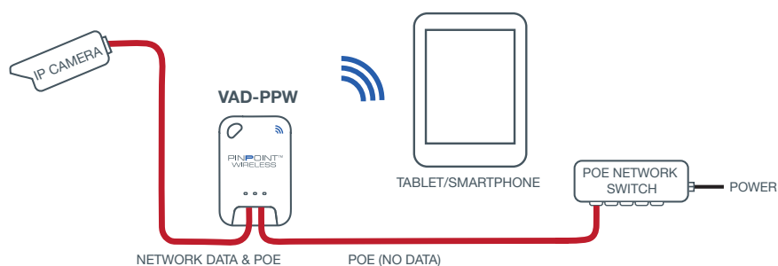
Diagram 1. PINPOINT Wireless connected in series with the IP camera provides a wireless link to a Smartphone or tablet
